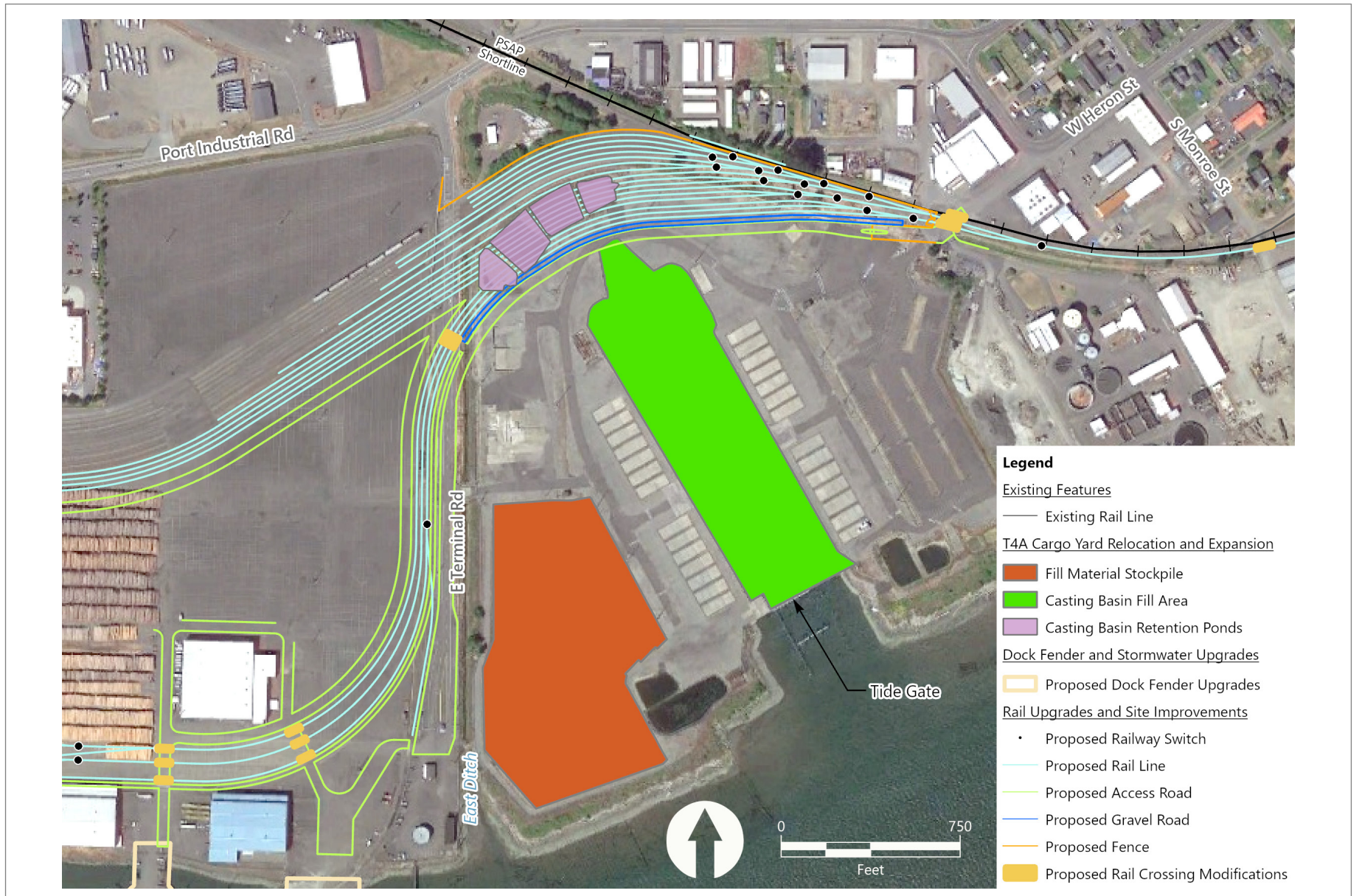
Figure 5 Terminal 4A Cargo Yard
