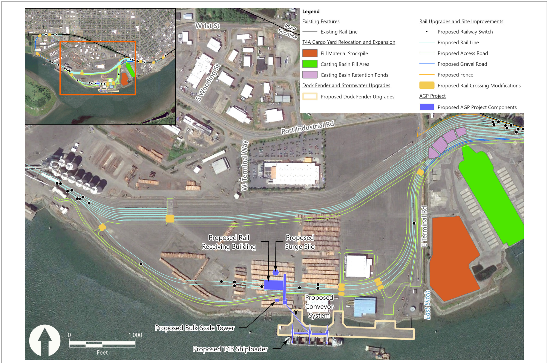
Figure 4b Rail Upgrades
