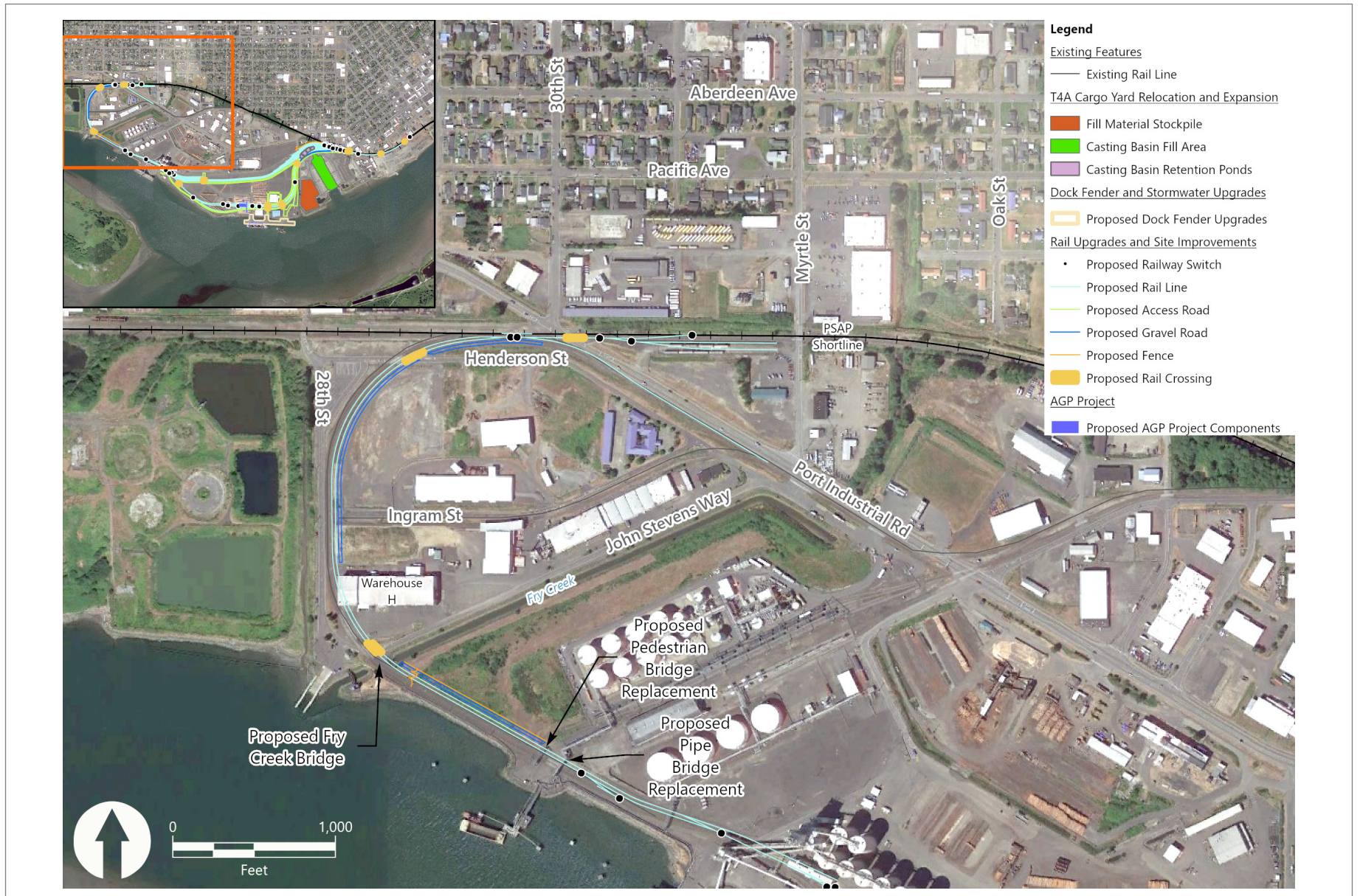
Figure 4a Rail Upgrades
